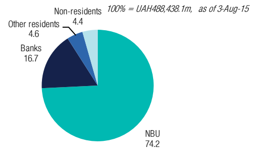
Chart 8. Domestic sovereign debt (%) as of 31 Jul 2015
