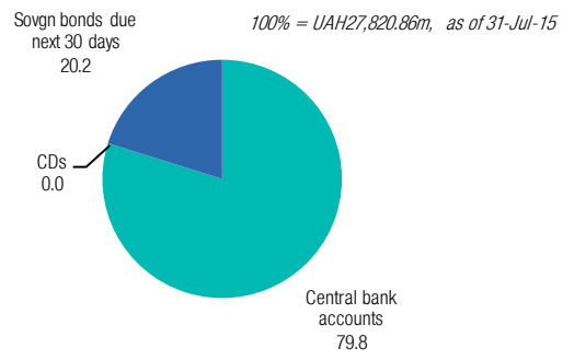
Chart 6. Breakdown of liquidity pool (%) as of 31 Jul 2015
