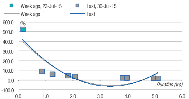
Chart 4. USD sovereign yield curve (%) as of 31 Jul 2015
